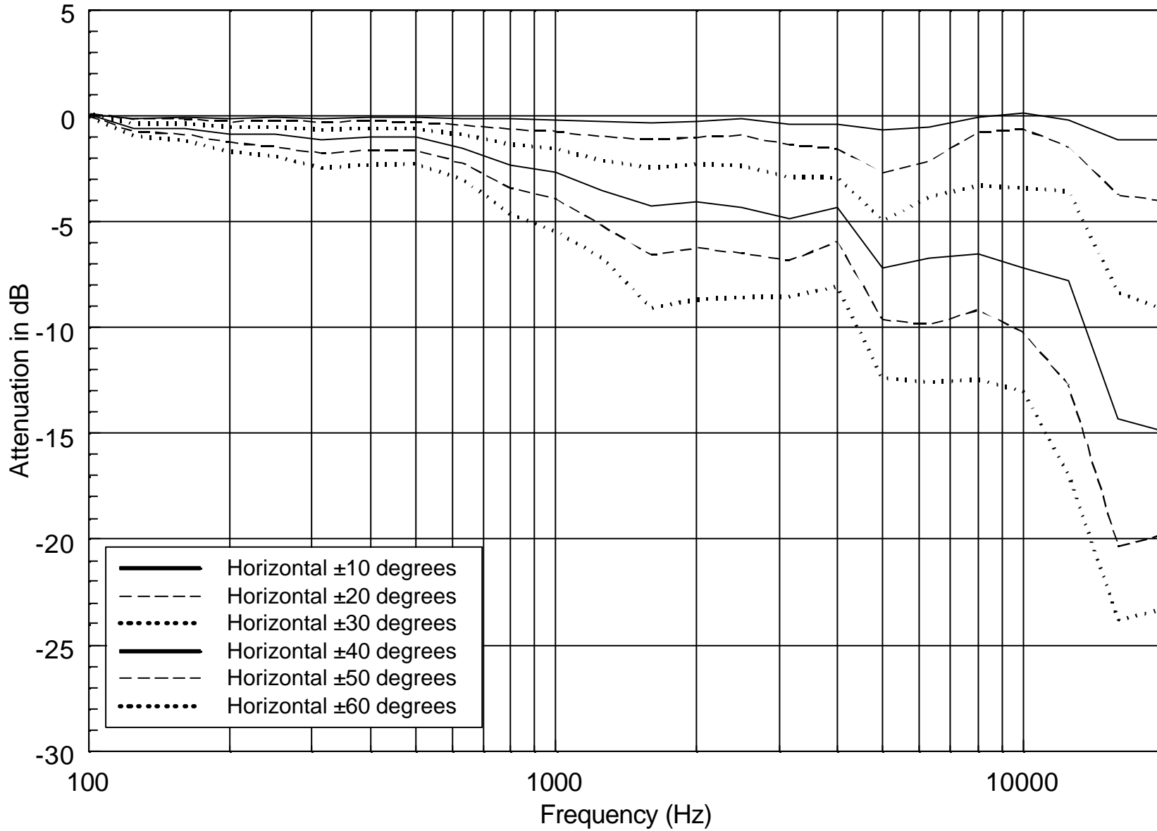
Normalized Horizontal off-axis Response
