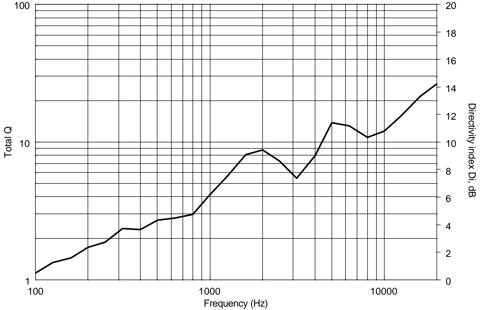
Directivity Index and Q
