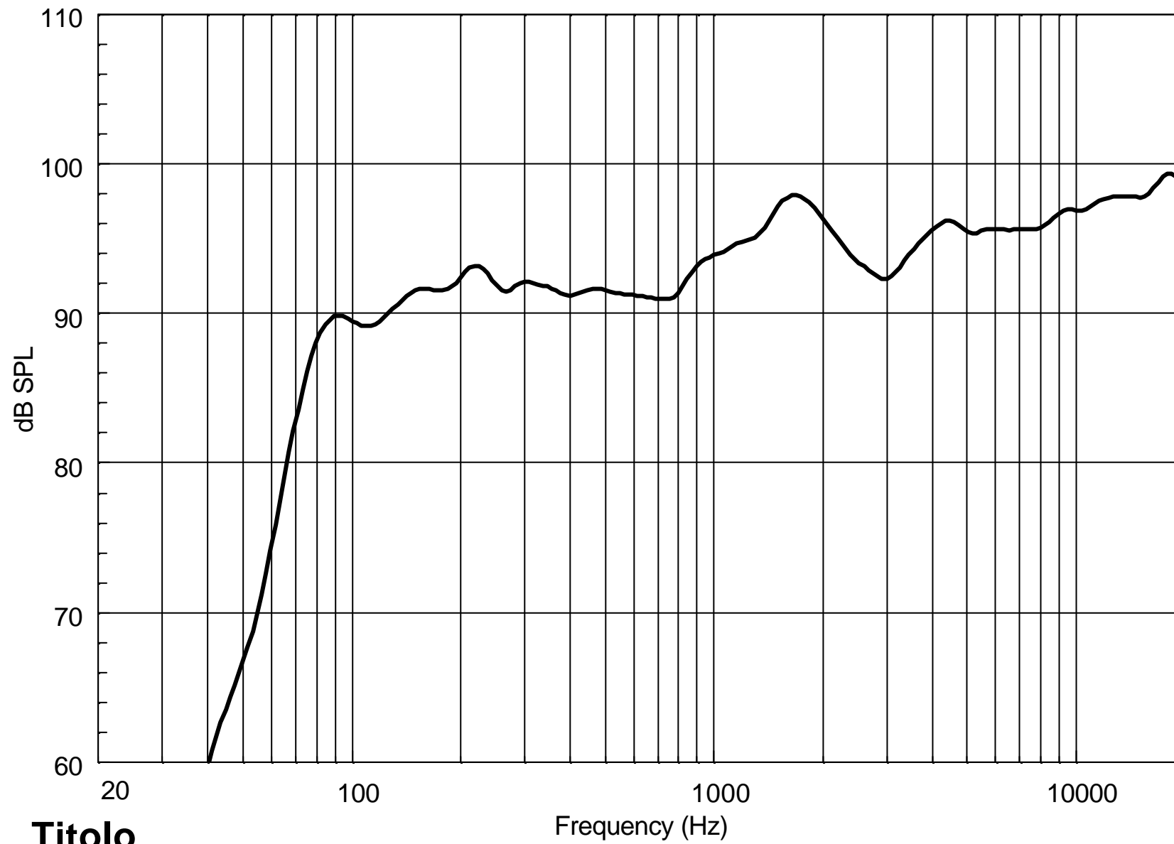
Response 1W/1m
