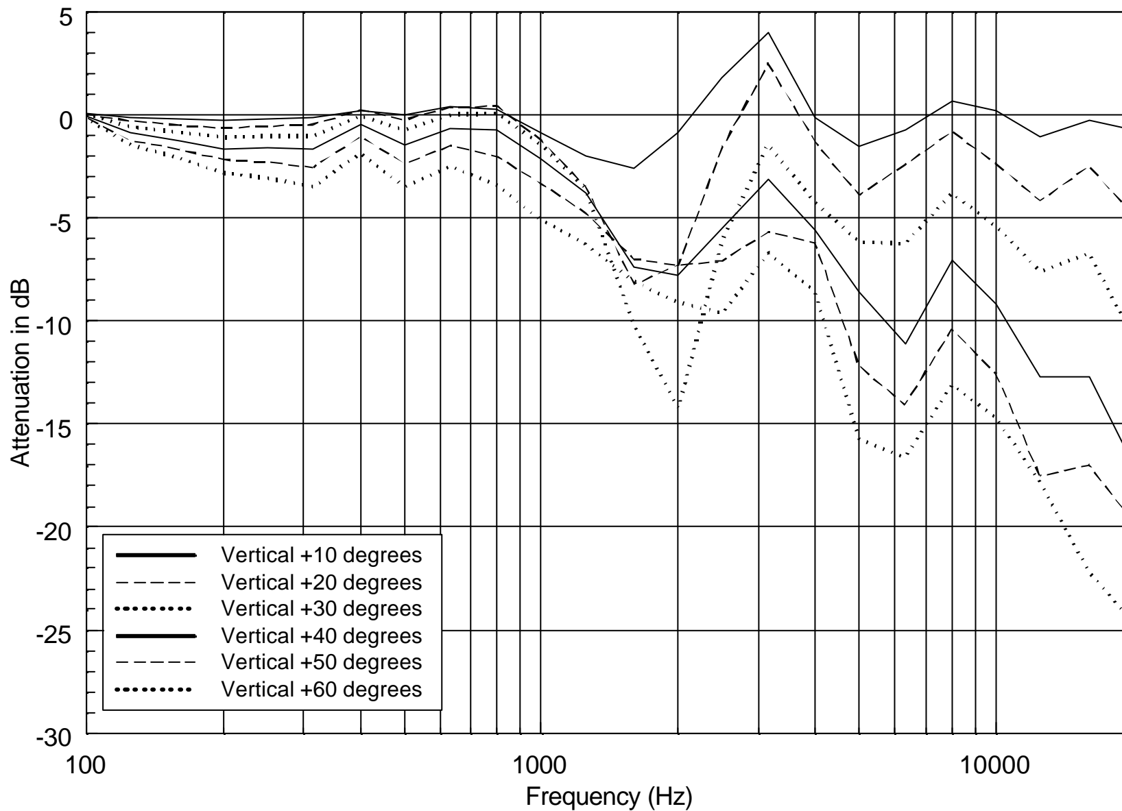
Normalized Vertical off-axis Response. Above the box
