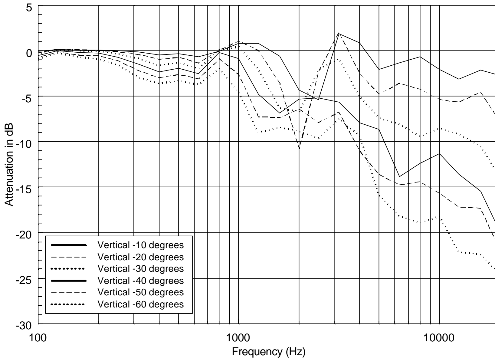
Normalized Vertical off-axis Response. Below the box
