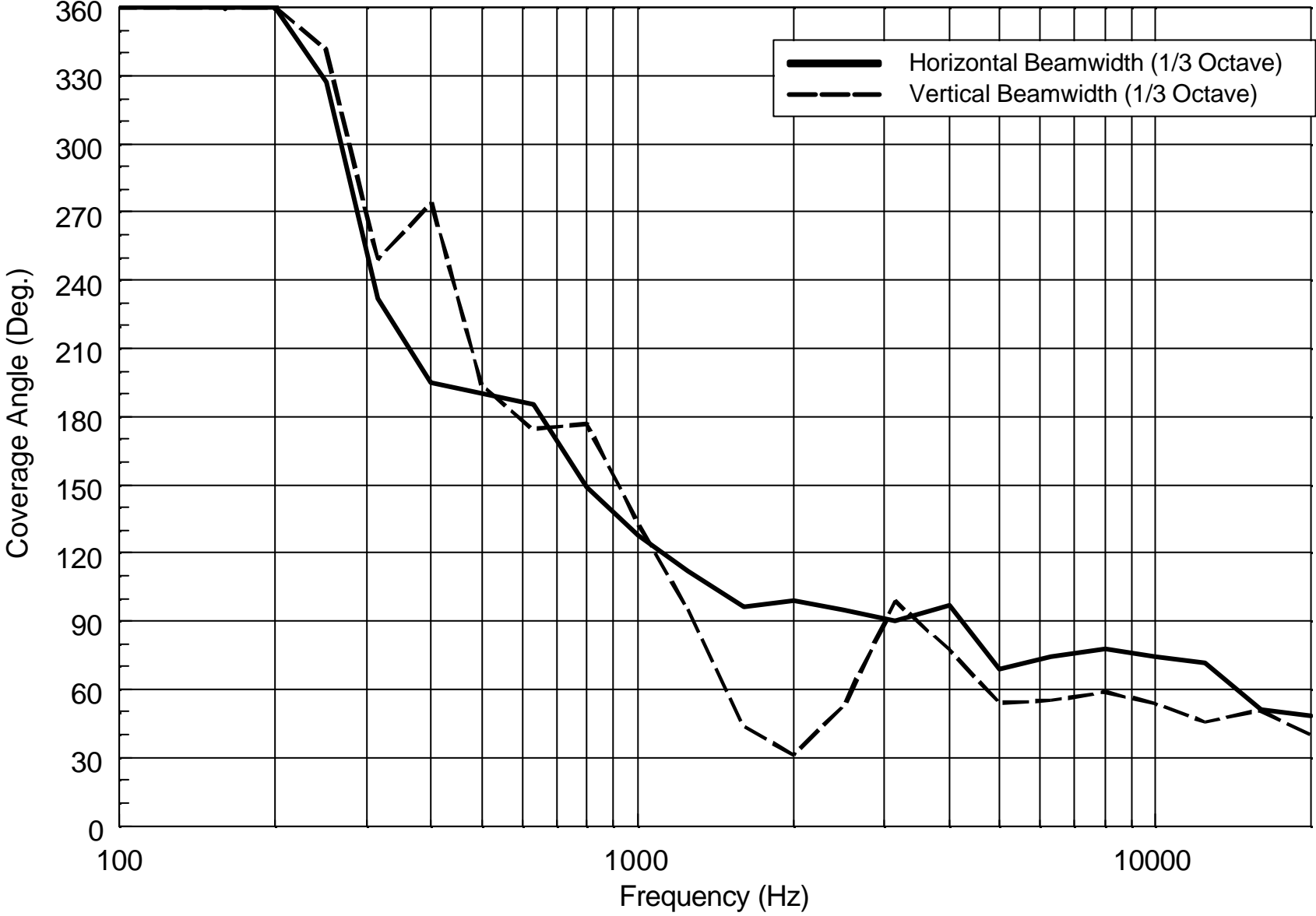
Beamwidth vs. Frequency
